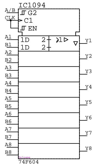
74F604 IC????
