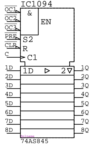
74AS845 IC????
