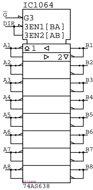
74AS638 IC????
