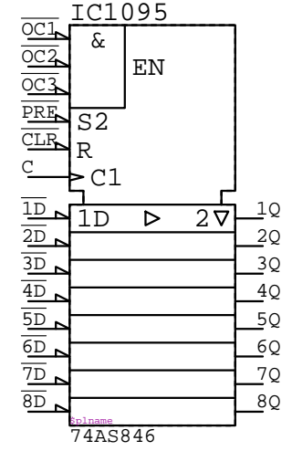
74AS846 IC????
