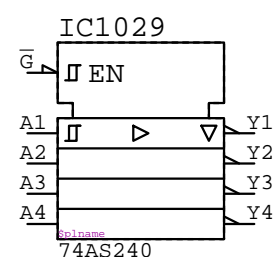
74AS240 IC????
