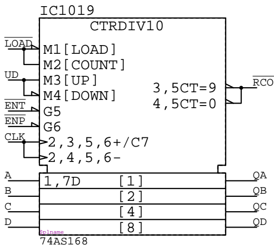
74AS168 IC?????
