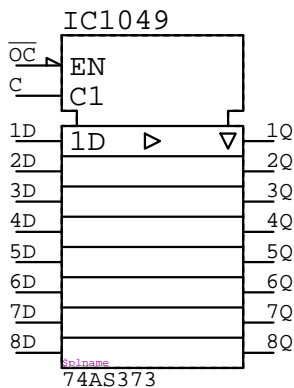
74AS373 IC?????
