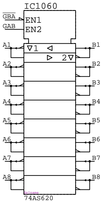
74AS620 IC????
