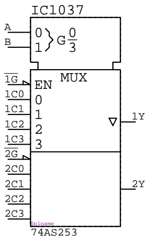
74AS253 IC????
