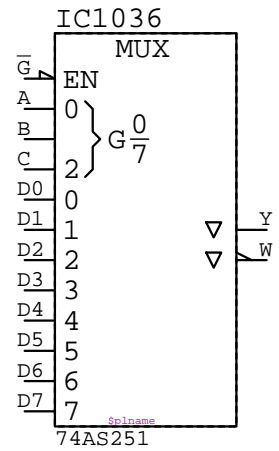
74AS251 IC????
