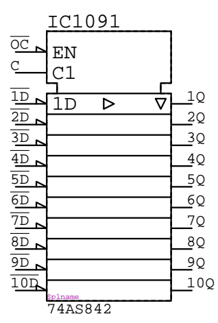
74AS842 IC????
