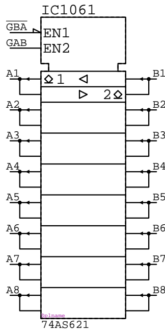
74AS621 IC????
