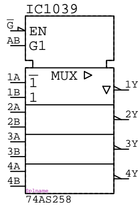
74AS258 IC????
