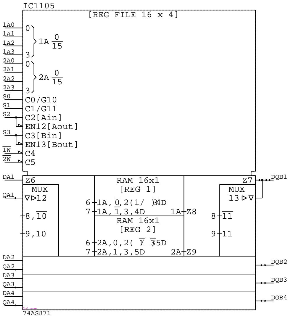
74AS871 IC????
