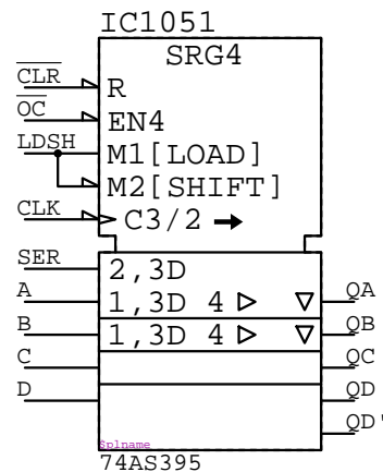
74AS395 IC?????
