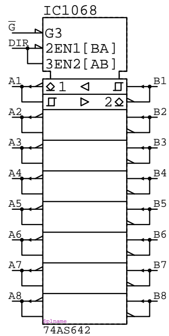
74AS642 IC????
