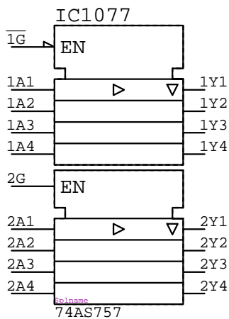
74AS757 IC?????
