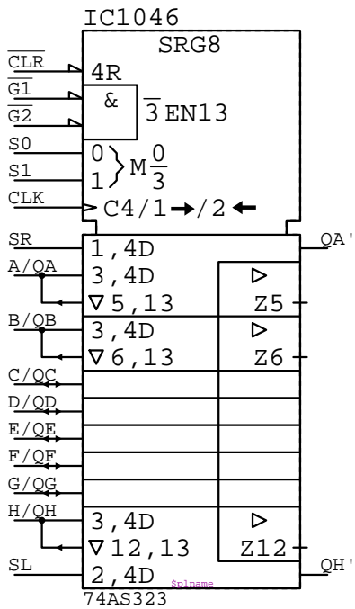
74AS323 IC?????
