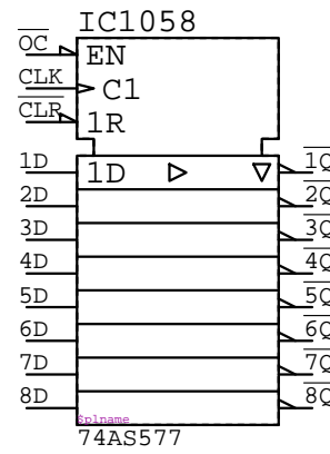
74AS577 IC????
