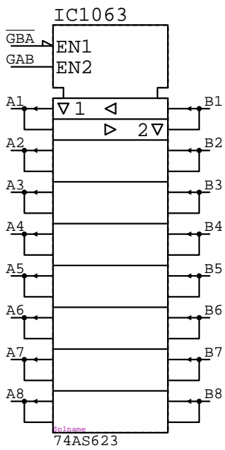
74AS623 IC????
