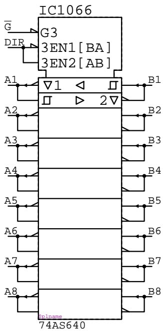
74AS640 IC????
