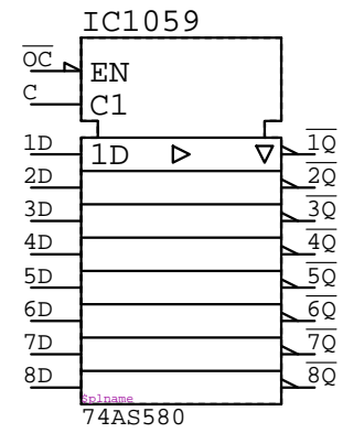
74AS580 IC????
