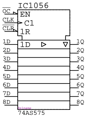
74AS575 IC????
