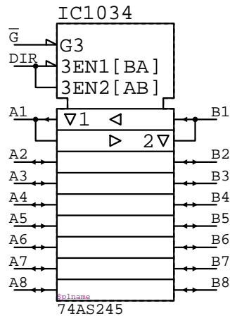
74AS245 IC????
