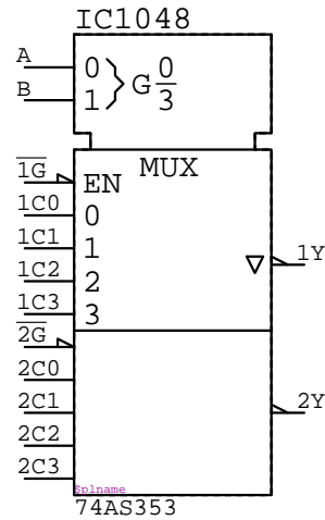
74AS353 IC?????
