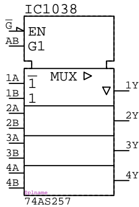
74AS257 IC????
