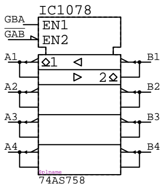
74AS758 IC?????
