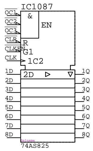
74AS825 IC????
