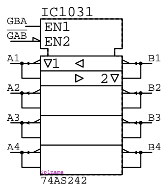
74AS242 IC????
