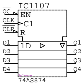
74AS874 IC????
