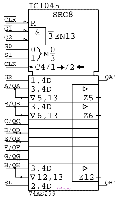
74AS299 IC?????
