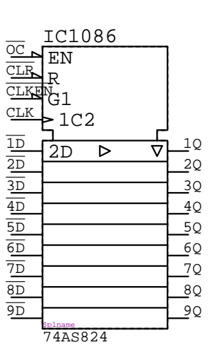
74AS824 IC????
