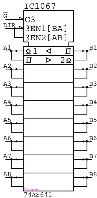
74AS641 IC????
