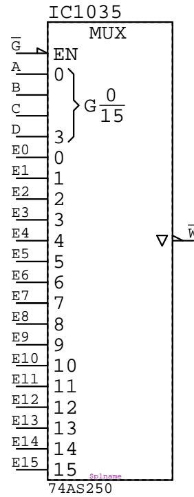
74AS250 IC????
