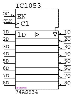
74AS534 IC?????
