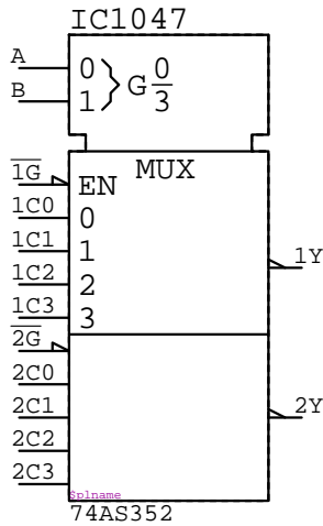
74AS352 IC?????
