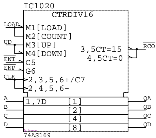
74AS169 IC?????
