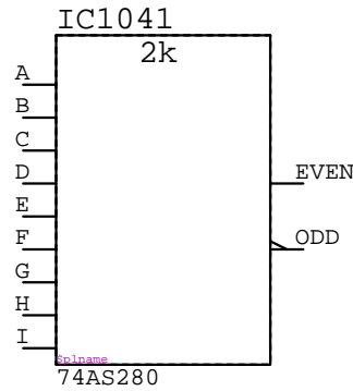
74AS280 IC?????
