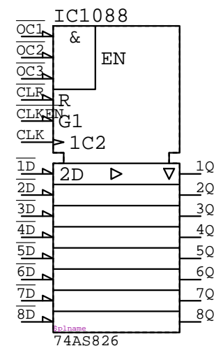
74AS826 IC????
