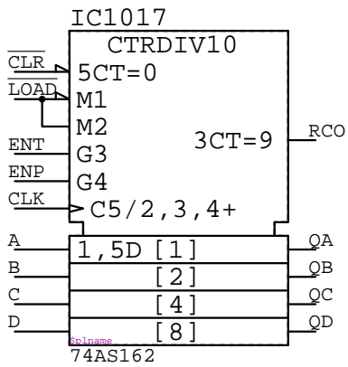
74AS162 IC?????
