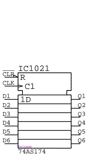
74AS174 IC?????
