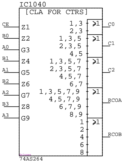
74AS264 IC?????
