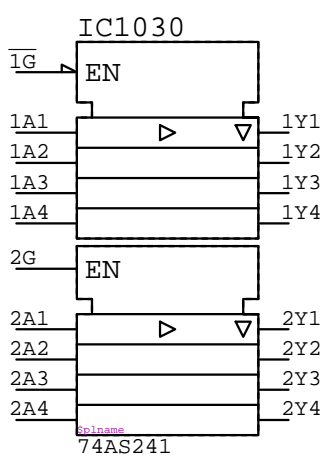
74AS241 IC????
