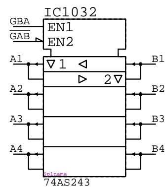
74AS243 IC????
