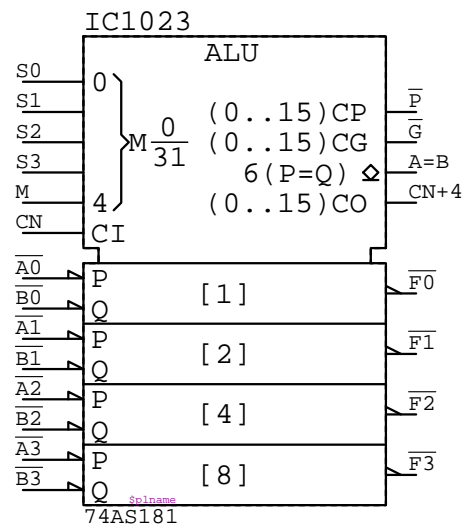
74AS181 IC?????
