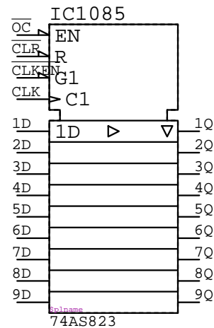
74AS823 IC????
