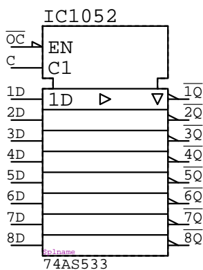
74AS533 IC?????
