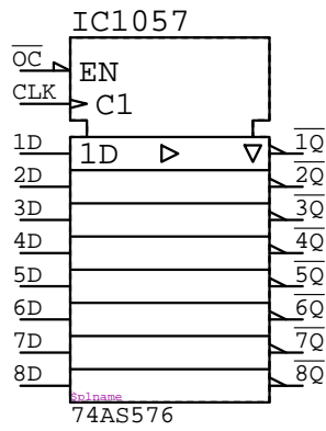
74AS576 IC????
