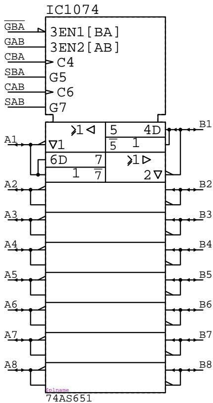
74AS651 IC?????
