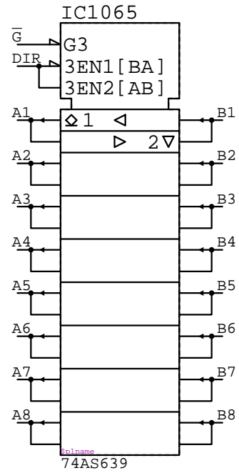
74AS639 IC????
