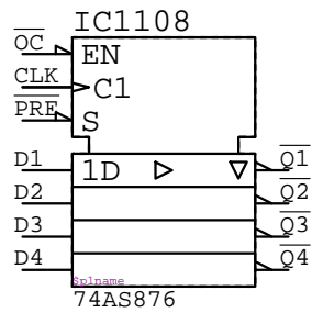
74AS876 IC????
