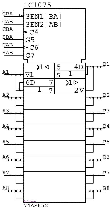
74AS652 IC?????
