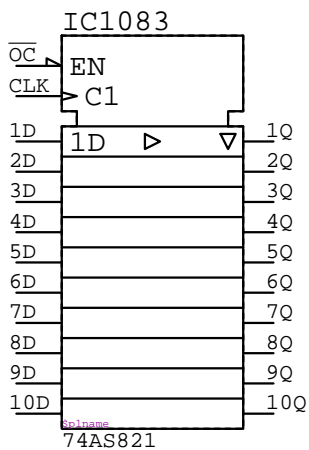
74AS821 IC????
