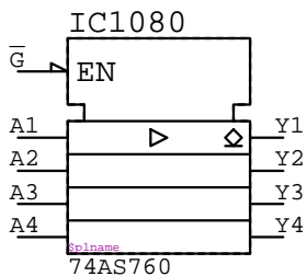
74AS760 IC?????
