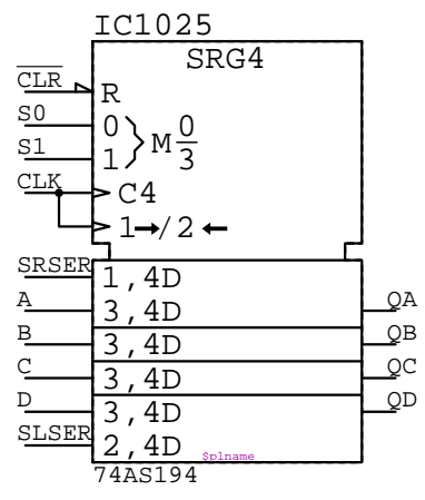
74AS194 IC????
