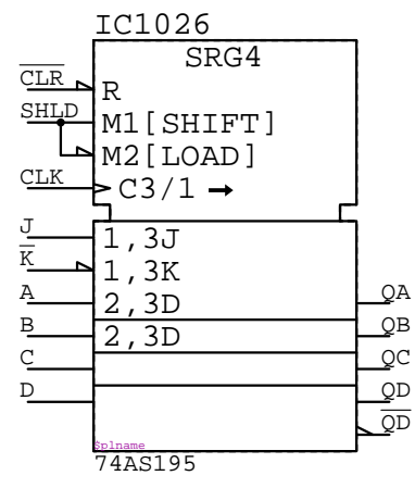
74AS195 IC????
