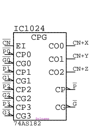
74AS182 IC????
