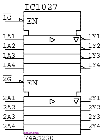
74AS230 IC????
