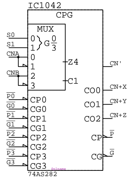
74AS282 IC?????
