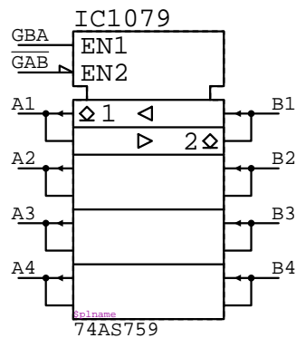
74AS759 IC?????
