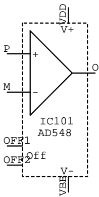
AD548 IC???
