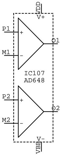
AD648 IC????
