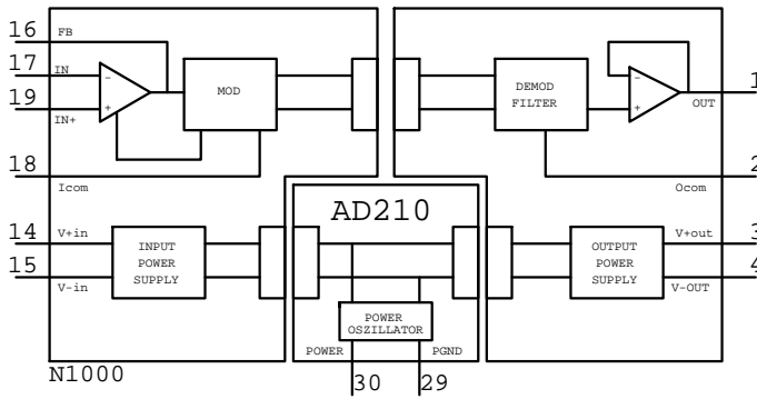
AD210 N????
