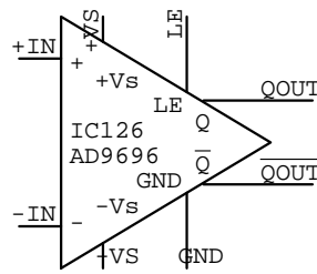
AD9696 IC???
