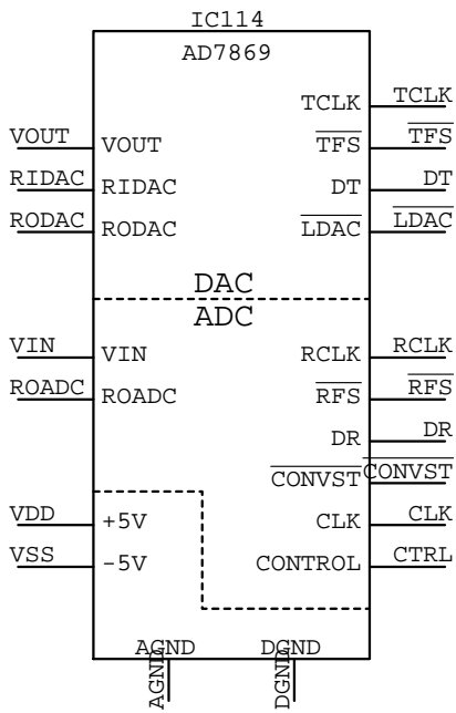
AD7869
