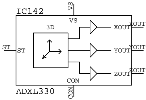
ADXL330 IC???
