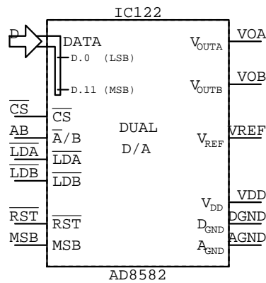
AD8582 IC???
