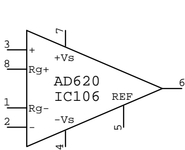
AD620 IC???
