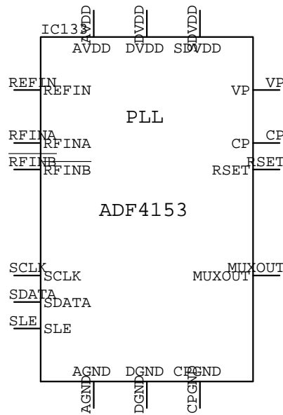
ADF4153
