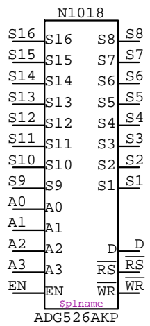
ADG526AKP N????
