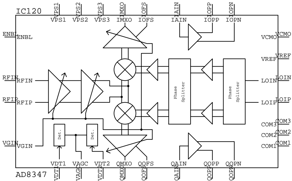
AD8347 IC???
