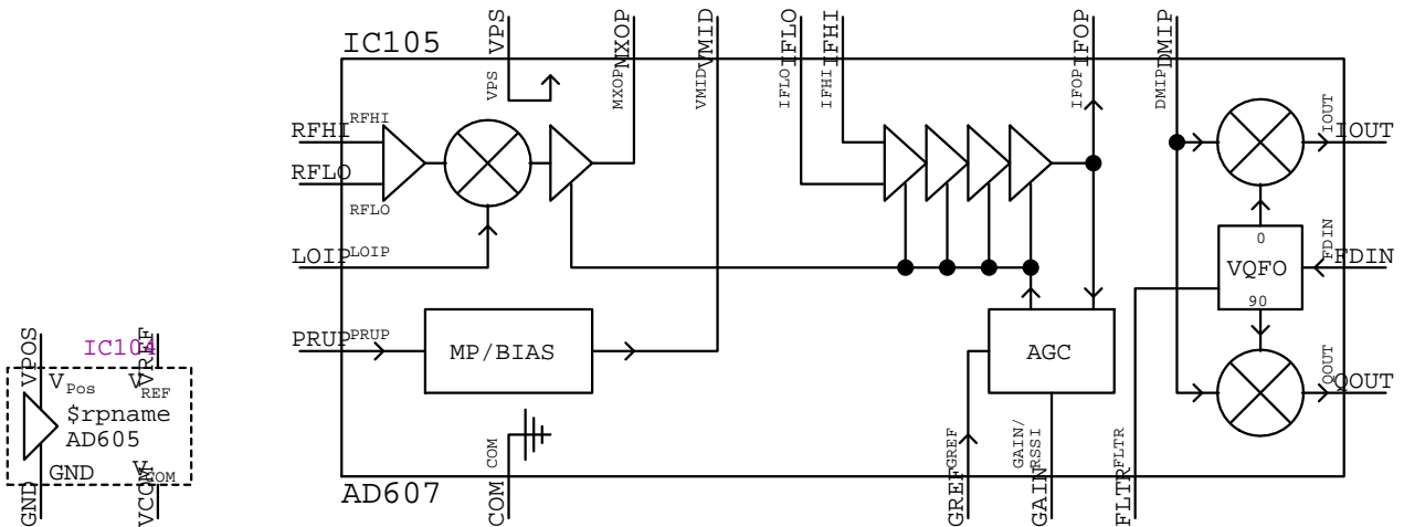
AD605_SUP IC???
