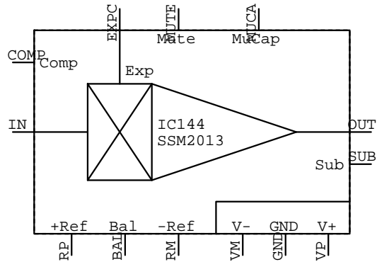
SSM2013 IC???
