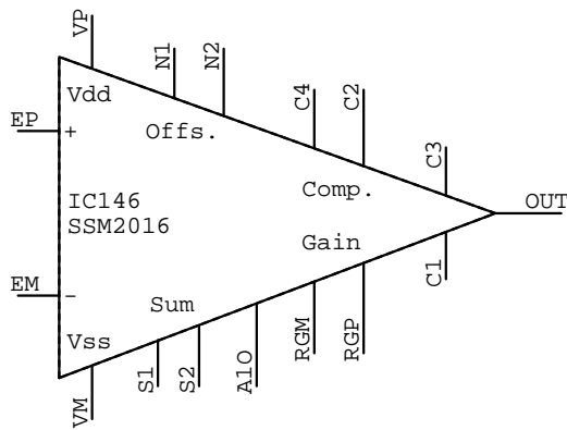
SSM2016 IC???
