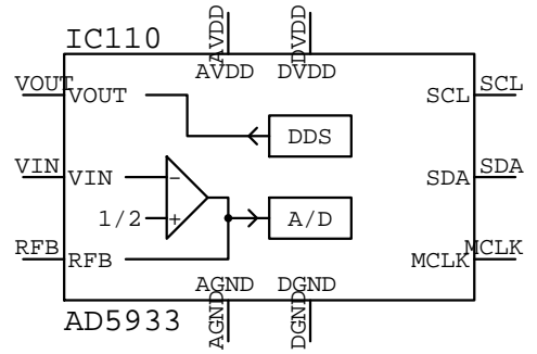
AD5933 IC????
