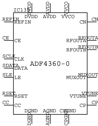
ADF4360_0
