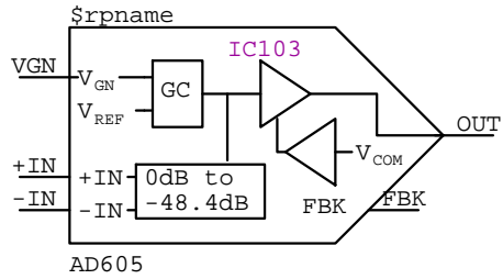
AD605 IC???
