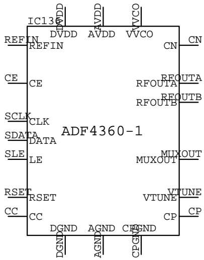
ADF4360_1 IC????
