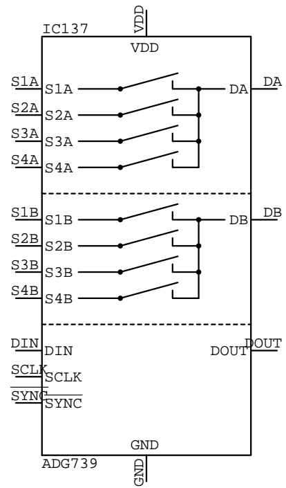
ADG739 IC???
