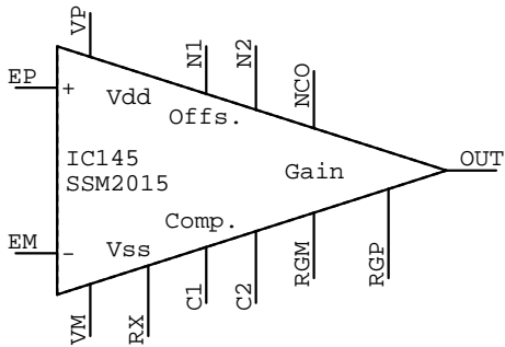
SSM2015 IC???
