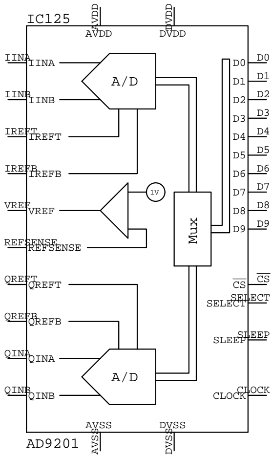
AD9201 IC???
