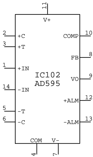
AD595 IC???
